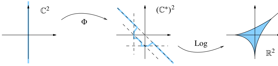
Figure 7: Amoeba with thin legs.
