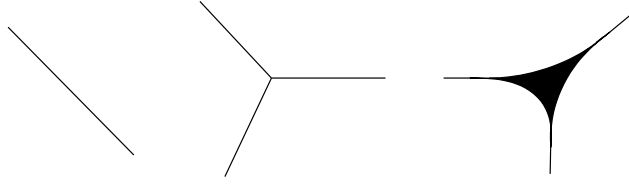
Figure 1: Components of \Delta , n = 3 .
