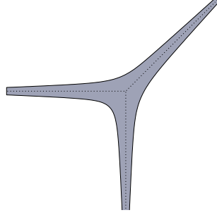
Figure 5: Amoeba of v_1 + v_2 + 1 = 0
