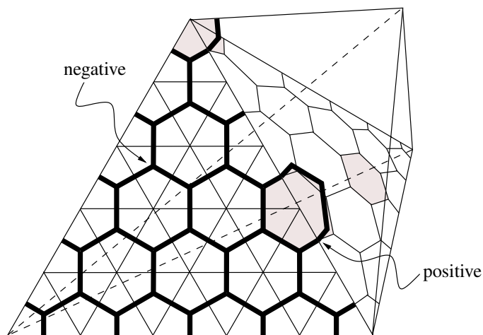
Figure 3: Affine S^3 with singularities.
