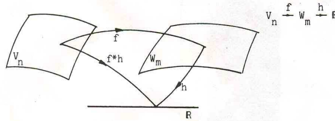
Figure 3: Diagrammatic representation of the pullback operation.
