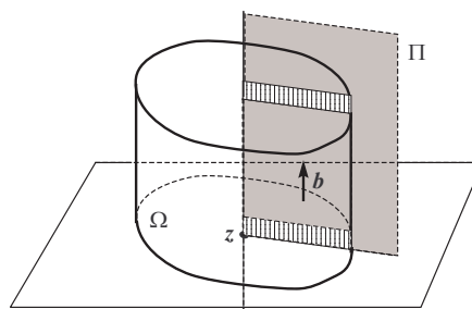
Figure 1: A screw Volterra dislocation in the cylinder \Omega \times \mathbb{R} .
